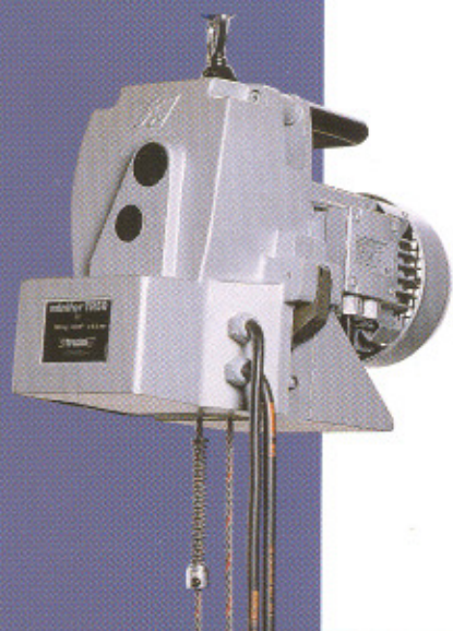
Minifor® TR30S - TR50 WLL 300 kg and 500 kg
