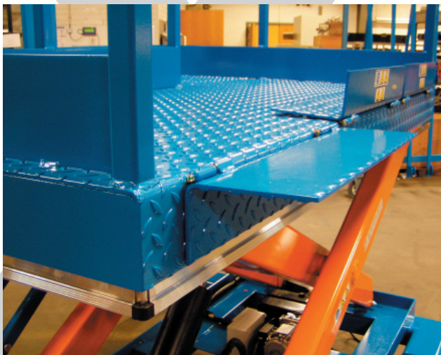
Platform extension flap.
